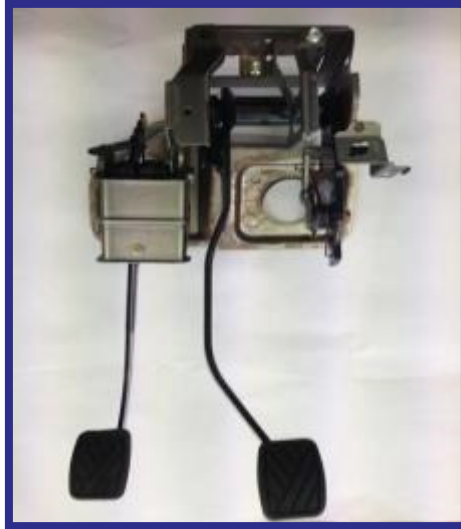
Pedal Box
